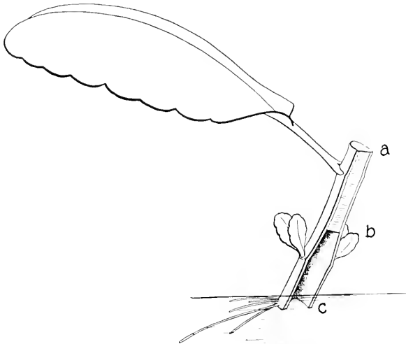
FIG. 114.—Proof that roots can be formed by cortex alone. Oct. 16 to Nov. 8, 1923.
